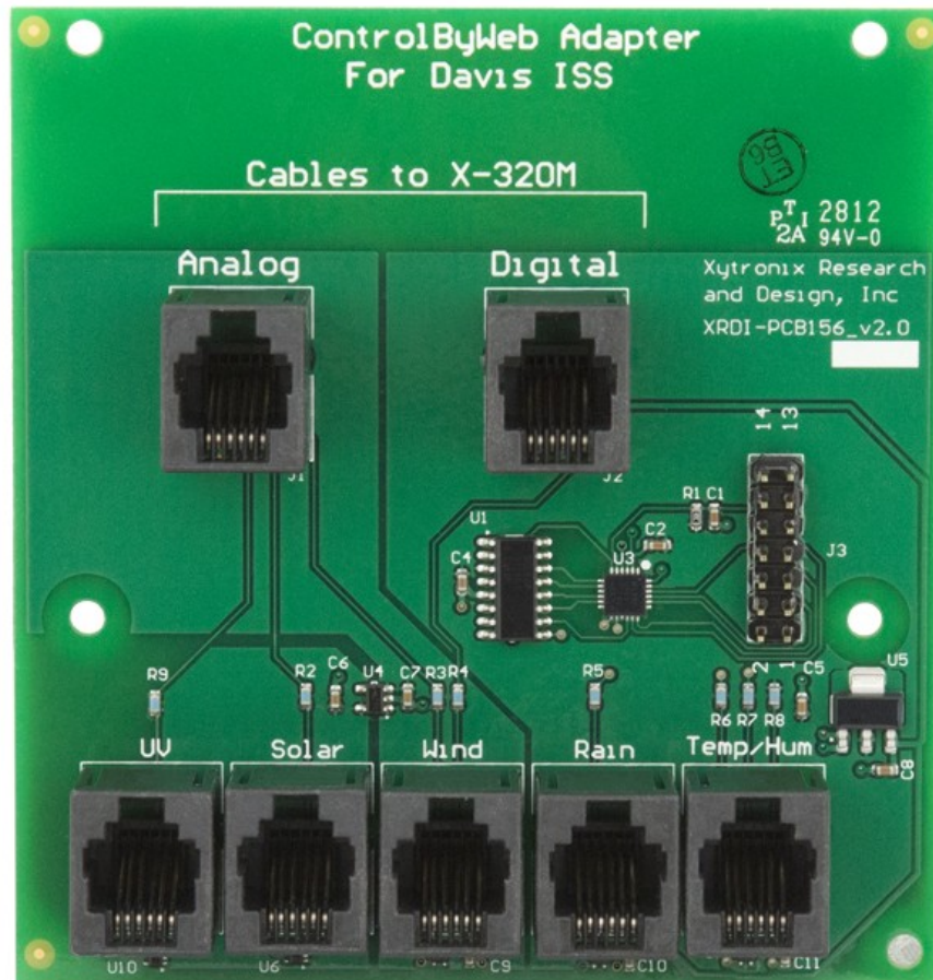
Figure 2: Davis Adapter Board
